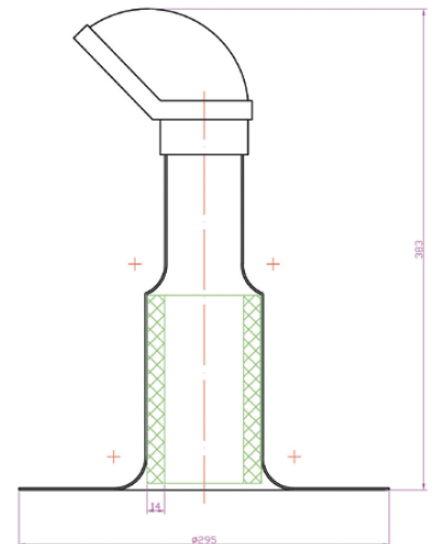
Fig. 1. Muti-Wire Insulated Cobra Head Electrical Flashing
